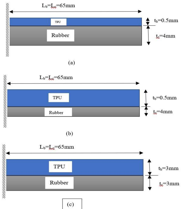
Fig.5: Specimens used in modelling
