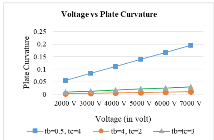
Fig.7: Voltage vs Plate Curvature on varying thickness of material
