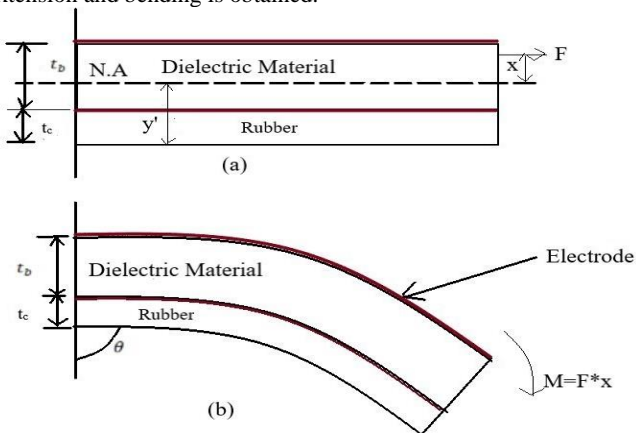
Fig.3: (a) Schematic diagram of two layer beam having TPU and Rubber
