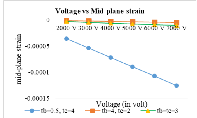
Fig.6: Voltage vs Mid plane Strain on varying thickness of materials
