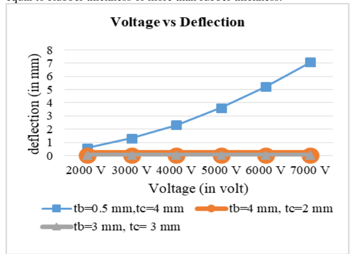
Fig.8: Voltage vs bending deflection graph
