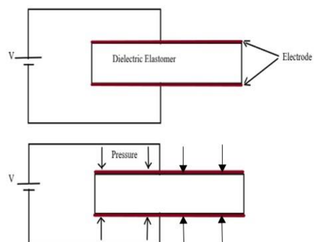
Fig. 1: Schematic diagram of Dielectric elastomer (a) Not in active state (b) activated state
